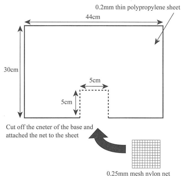
Fig. 2. Schematic diagram of the pupation-site trap
