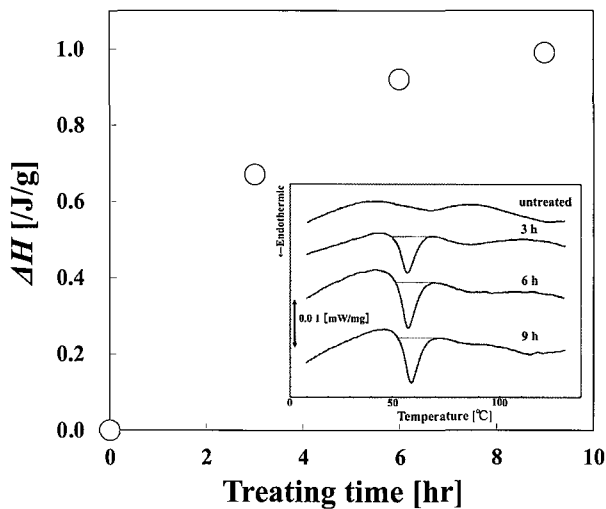
Fig. 2 DSC curves of untreated rice flour and ball-milled rice flour and dependence of \Delta H on ball milling time.
