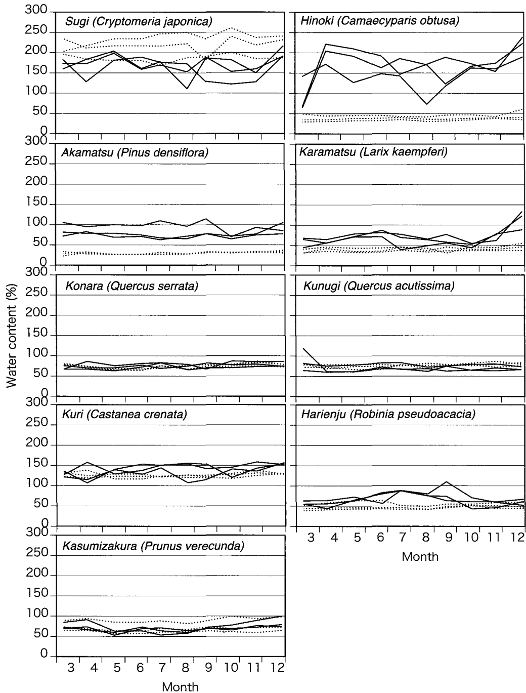
Fig. 2. Seasonal changes in water content of sapwood (lines) and heartwood (dotted lines) for 9 species.
