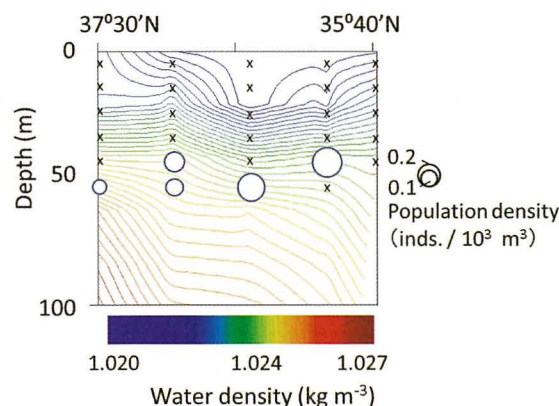
Fig. 47. Vertical distribution of N. nomurai with water density contour on 133° 30' East longitude (September 2009).
