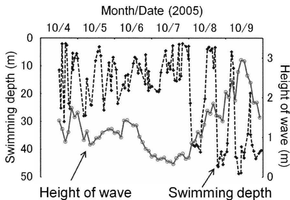
Fig. 59. Time series data of wave height and swimming depth of a N. nomurai . Swimming depth was investigated by Pop-up archival tag (PAT5, Bell diameter: 1.5 m).
