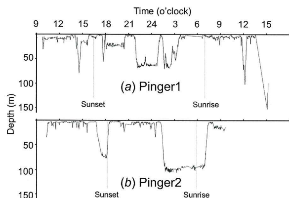
Fig. 33. Time-series data of swimming depths of N. nomurai investigated using pingers.
