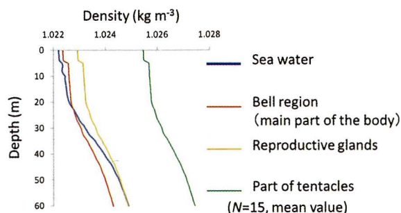
Fig.48. Density of the seawater and body parts of N. nomurai with depth (Mean value of 15 individuals, September 2009).
