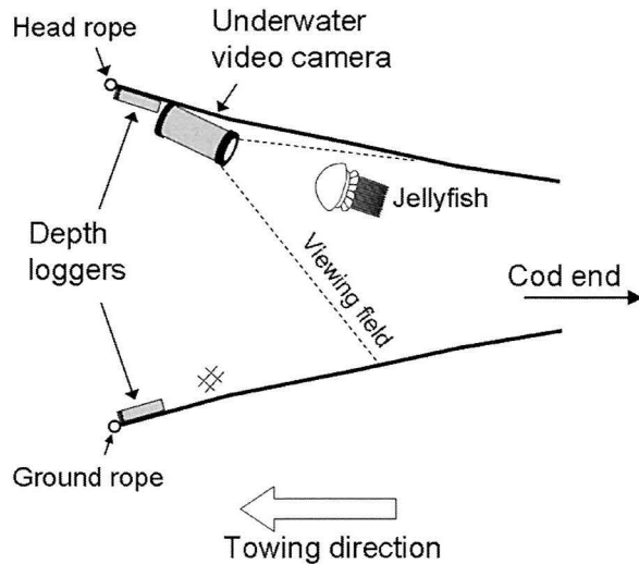
Fig. 22. Sectioned diagram of an underwater video camera and depth loggers mounted in LC-V small trawl net.
