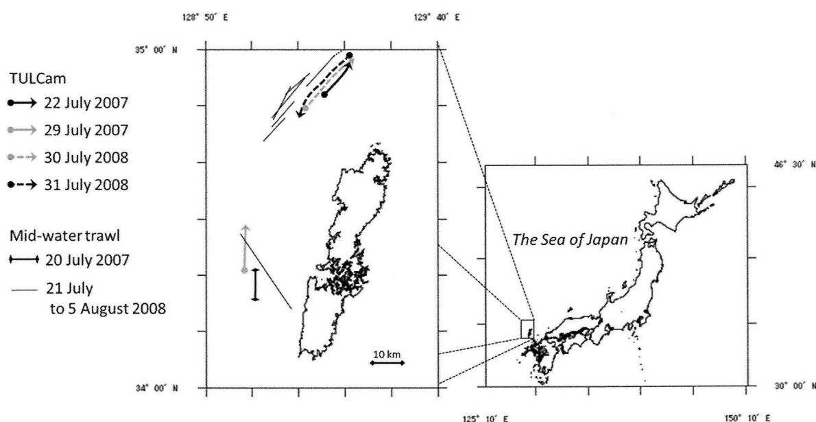
Fig. 7. Experimental area and survey lines in the Western Channel of the Tsushima Strait in the Sea of Japan. Arrows directions indicate towing directions in TULCam surveys.
