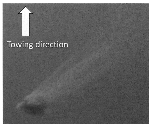
Fig. 16. An example picture of Cyanea nozakii observed by TULCam at the depth of approximately 50 m.
