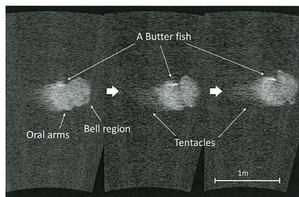
Fig. 39. Sequence images of N. nomurai and a Butter fish Psenopsis anomala taken with an acoustic camera operated by 1.8 MHz (about 4 m distance from DIDSON). A bell of the jellyfish was opening gradually in these pictures. A remarkably white shadow is a Butter fish.
