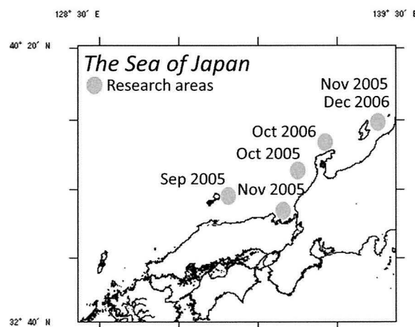
Fig.2. Research areas and date in the Sea of Japan.
