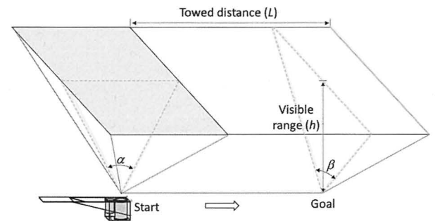
Fig. 6. Schematic drawing of observed water volume by TULCam observation.
