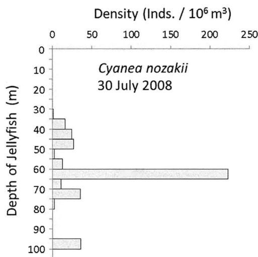
Fig. 18. Vertical distribution of depth of C. nozakii estimated by TULCam survey on 30th July 2008 ( N = 46 ).
