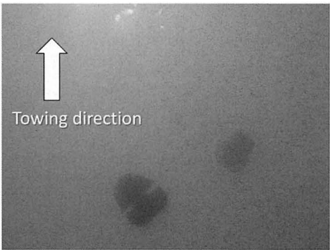
Fig. 13. An example picture of N. nomurai observed by TULCam at the depth of approximately 20 m. The white dots above the jellyfishes on the picture are the sunshine-glare on the sea surface. Arrow direction indicates towing direction of TULCam.
