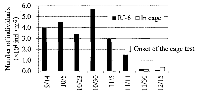
Figure 6. Density of Manila clam population in RJ-6 and cage test from September to December in 2015. Cage test was set on November 11, 2015.
