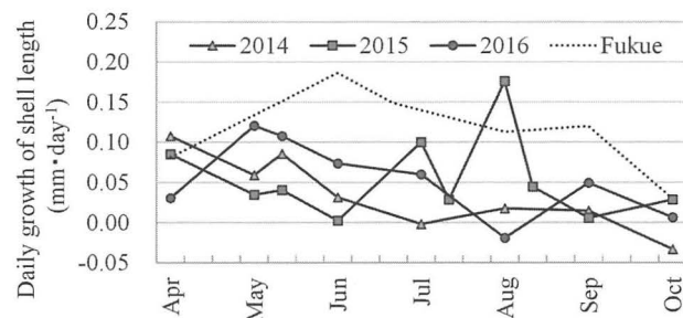
Figure 4. Seasonal changes of daily growth of Manila clams in RJ-2, 4, 6 and Fukue station (Aichi prefecture, 1983) from April to October in each year, 2014–2016.
