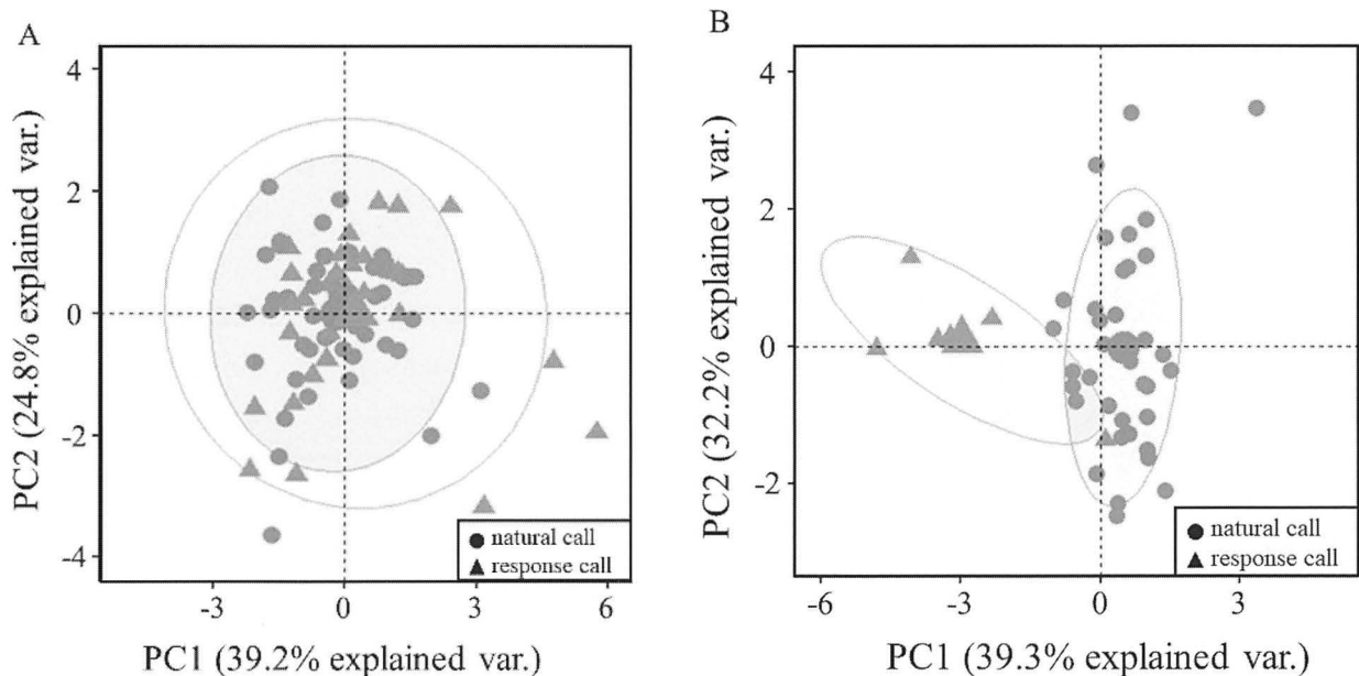
Fig. 2 Two-dimensional plots of PC1 vs. PC2 in natural and artificial settings. A : “Gururu” calls in the two different settings. B : “Kyokyo” calls in the two different settings. PC=principal component.
