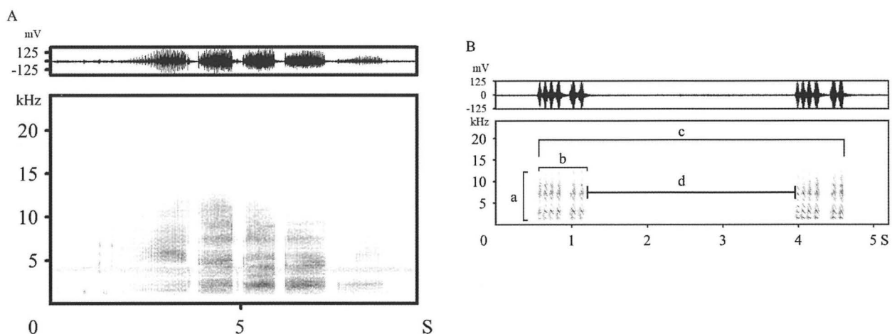
Fig. 1 Sound spectrograms of “Gururu” and “Kyokyo” recorded calls. A: “Gururu” recorded call for which the frequency range was between 1 kHz and 15 kHz. FFT size of 1024. B: “Kyokyo” recorded calls for which the frequency range was between 1 kHz and 12 kHz. FFT size of 512. The horizontal axis represents time (s) and the vertical axis represents the frequency (kHz). The call was recorded on Mt. Takao from a female individual. To reduce the background noise, we removed all sounds in the frequency range of 1 kHz. Call measurements are (a) peak frequency, (b) duration of the note, (c) duration of the call bout, and (d) inter-note interval.
