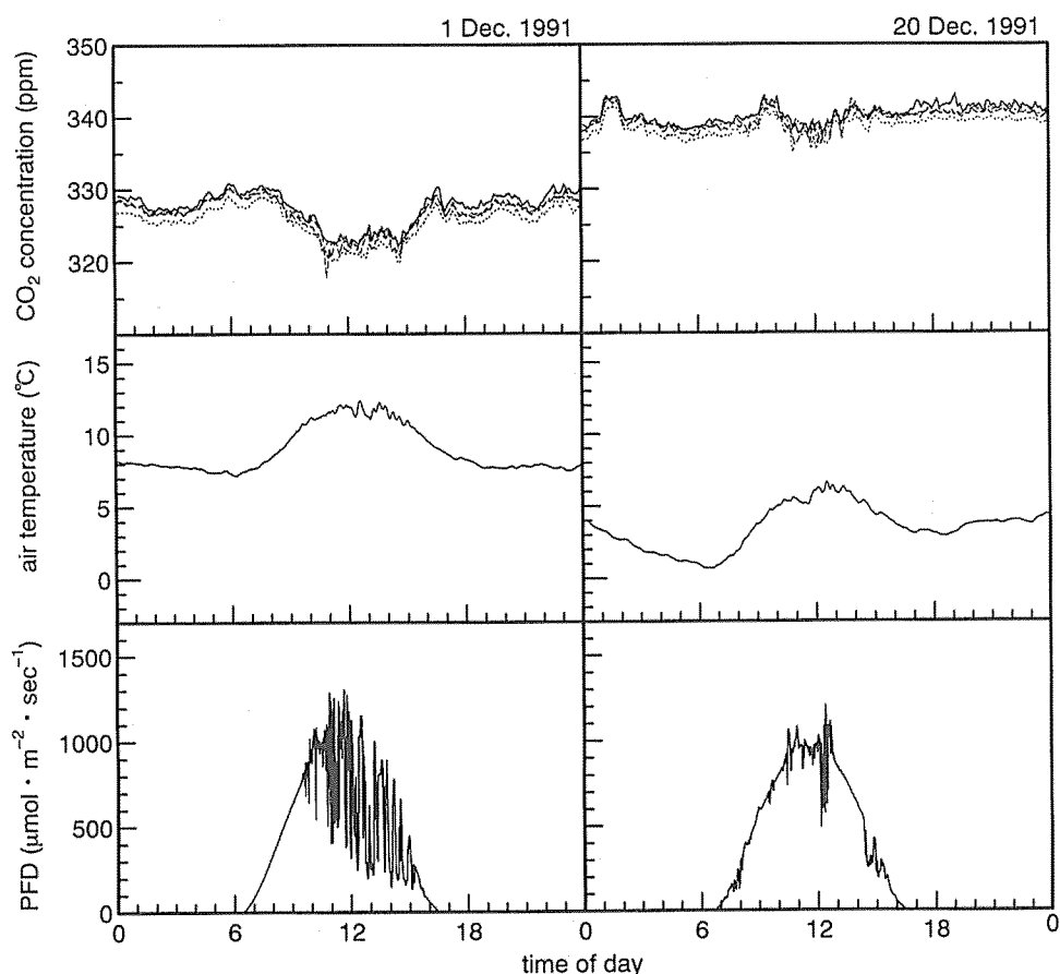
Fig. 5. Temperature effects on CO 2 concentrations within a Japanese cedar forest in winter. Top panels; CO 2 concentration, solid line; near the forest floor, dotted line; in the lower canopy, dashed line; in the upper canopy, dot dashed line; above the canopy. Middle panels; air temperature. Bottom panels; photon flux density (PFD) above the canopy.
