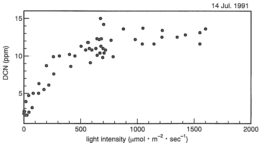
Fig. 4. The relationship between light intensity and daytime CO 2 concentration decrease from the daily nighttime level (DCN). Light intensity was given as the mean photon flux density for each one hour prior to the each CO 2 measurement time.
