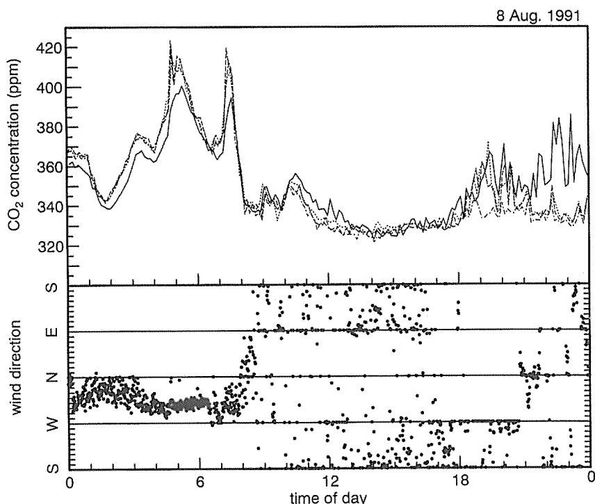
Fig. 6. Wind direction effects on CO 2 concentrations within a Japanese cedar forest. Solid line; near the forest floor, dotted line; in the lower canopy, dashed line; in the upper canopy, dot dashed line; above the canopy. Wind direction measured above the canopy were shown in the lower panel.
