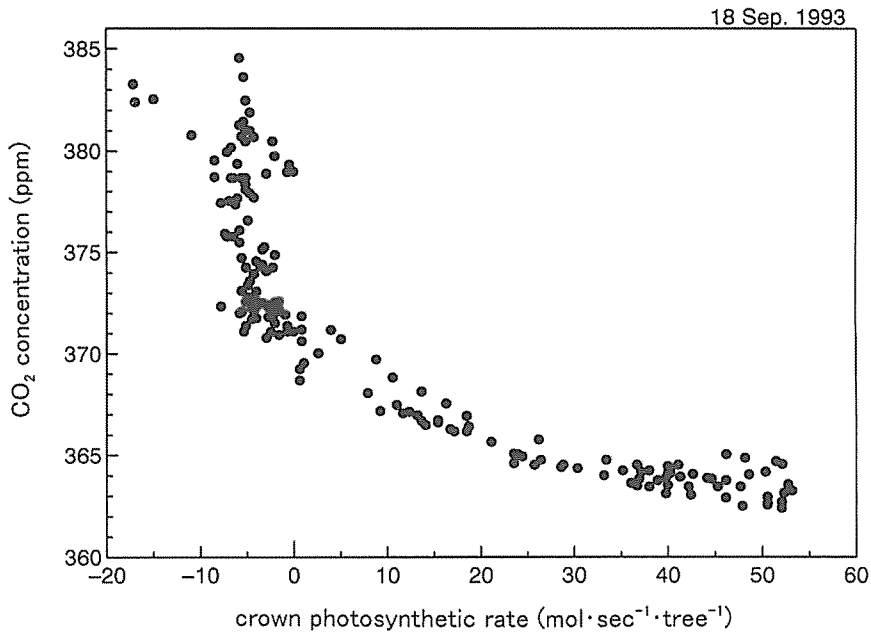
Fig. 3. Photosynthetic effects on CO 2 concentration within a Japanese cedar forest. Crown photosynthetic rates were measured with the crown chamber method.
