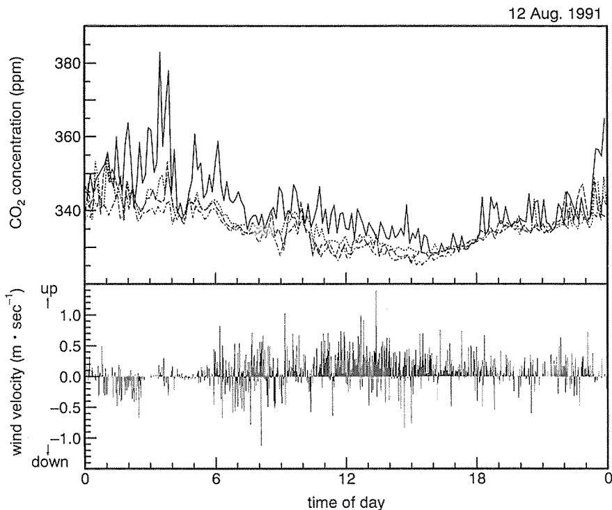
Fig. 1. Diurnal fluctuations of \text{CO}_2 concentrations at four heights within a Japanese cedar forest. Solid line; near the forest floor, dotted line; in the lower canopy, dashed line; in the upper canopy, dot dashed line; above the canopy. Vertical wind velocity measured above the canopy were shown in the lower panel.
