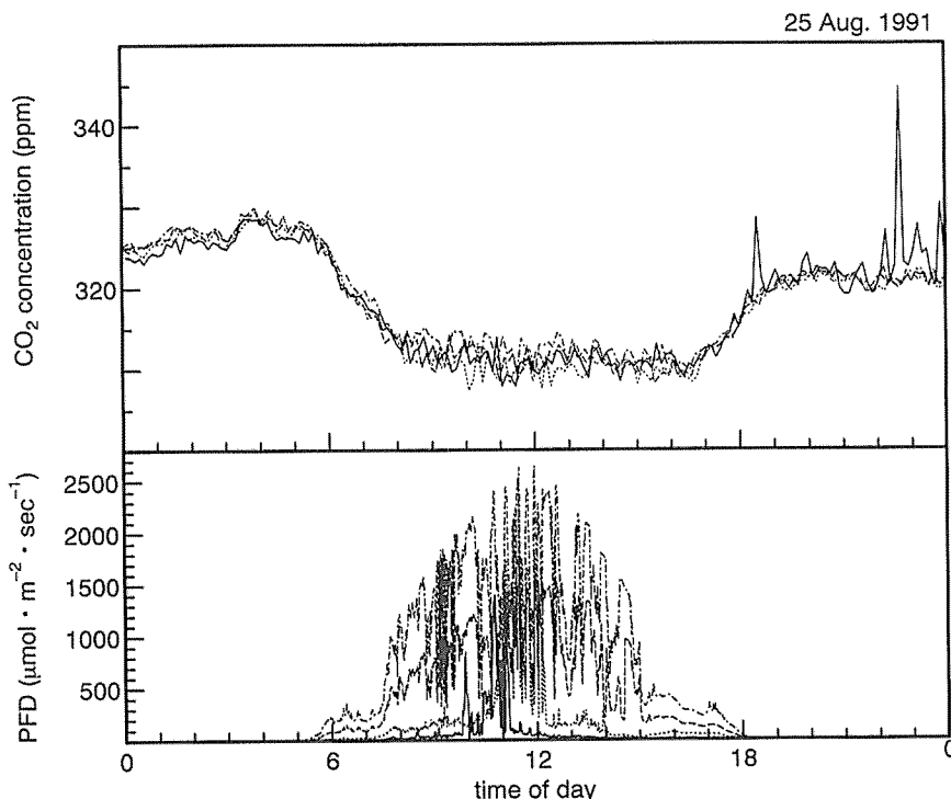
Fig. 2. Typical diurnal courses of CO 2 concentrations at four heights within a Japanese cedar forest on fair days in summer. Solid line; near the forest floor, dotted line; in the lower canopy, dashed line; in the upper canopy, dot dashed line; above the canopy. Photon flux density (PFD) at four heights are shown in the lower panel.
